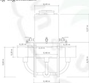
Gambar 5. Tampak “Wastafel Bundar”.
