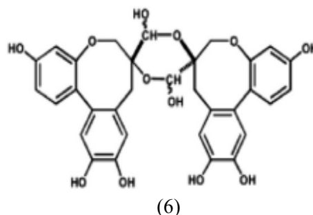
Figure 3. Molecular structure of Brazilin (1), Brasilein (2), Fangininoksi A (3), Fanginin A (4), Protosappanin D (5), Protosappanin (6) from C. sappan L.
