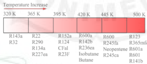
Fig. 3. Working fluids selection hint according to the heat sources temperature [59]
