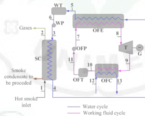
Fig. 4. Schematic flow diagram of the ORC integrated to smoke condensation process
