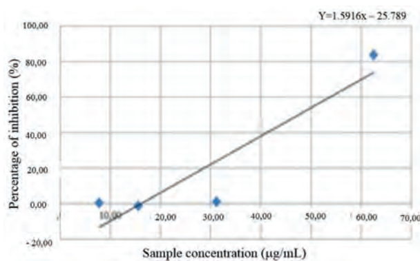
Figure 2. Curve results of L. ferrugineus Roxb acetone extract test against HeLa Cells.
