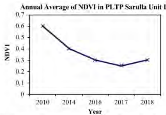
Figure 2. Graph of Average Change in NDVI at PLTP Sarulla Unit 1
