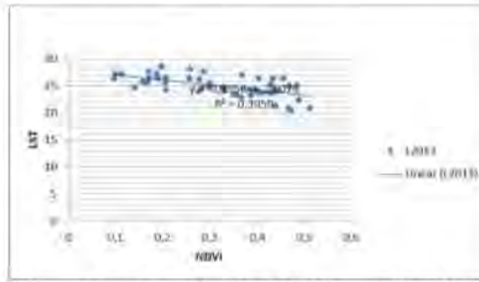
Figure 4.8 Relation Graphic of NDVI and LST in 2013
