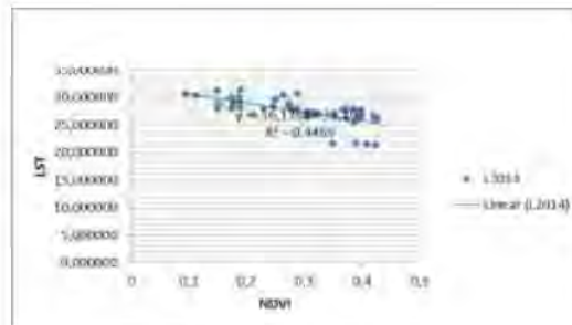
Figure 4.9 Relation Graphic of NDVI and LST in 2014
