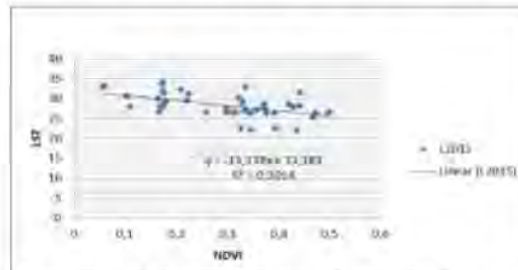
Figure 4.10 Relation Graphic of NDVI and LST in 2015
