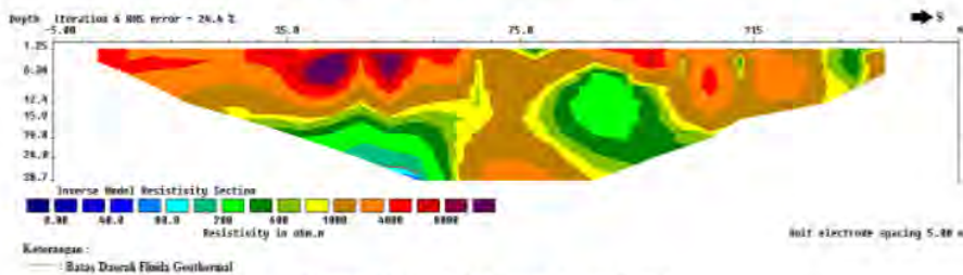
Figure 5. Resistivity section of line 3
