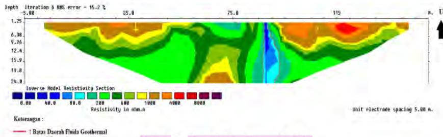
Figure 4. Resistivity section of line 2
