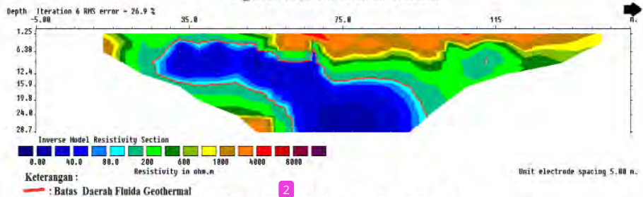
Figure 3. Resistivity section of line 1
