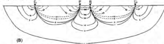
Figure 1. Schlumberger array sensitivity pattern plot
