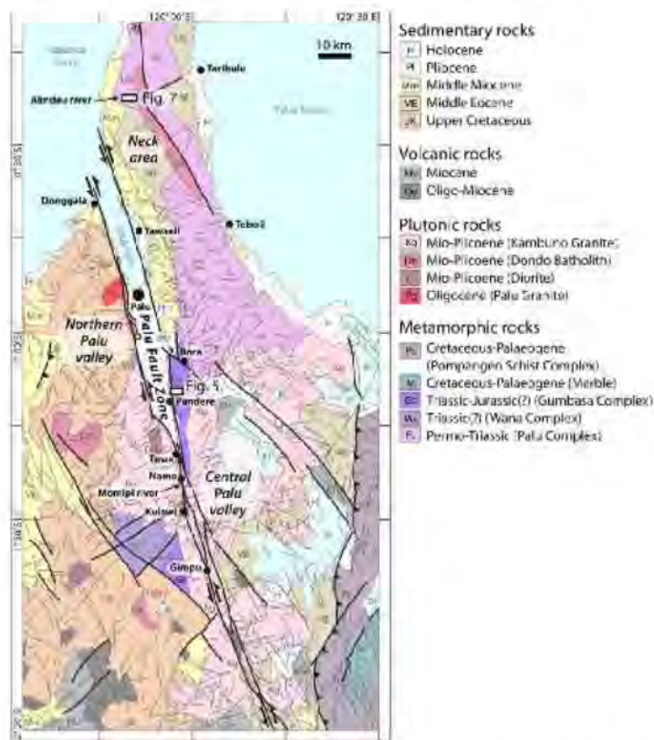
Figure 1. Geomorphologic and structural map of Palu-Koro fault lies on Sulawesi Island.
