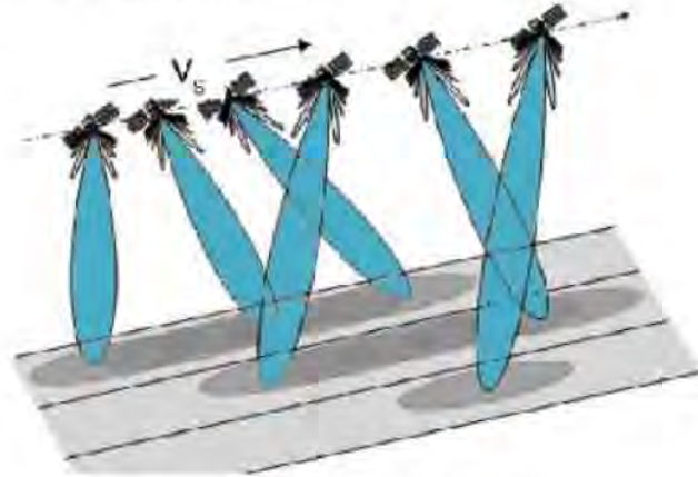
Figure 2. SAR Sub-Swath Acquisition
