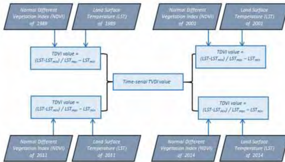
Figure2. TVDI Value in Coastal Area of Medan
