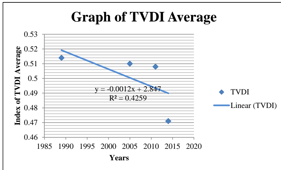
Figure 4. Graph of TVDI Average for 1989 - 2014
