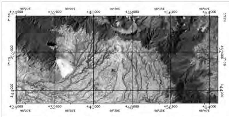
FIGURE 2. Mt. Sinabung in InfraRed Light (Band 10,6,5)
