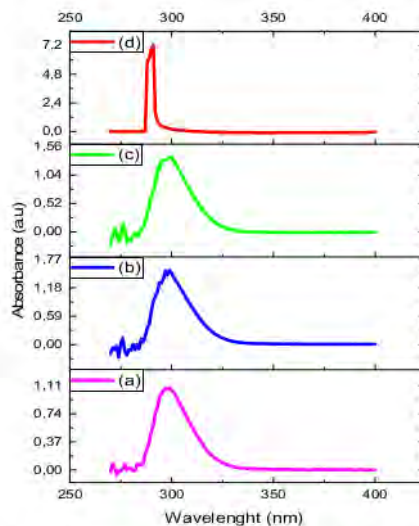
Fig.-4: Pattern of UV-Vis Absorbance Spectrum with Variations in Glutaraldehyde; (a) A1; (b) A4; (c) A5 and (d) Ar
