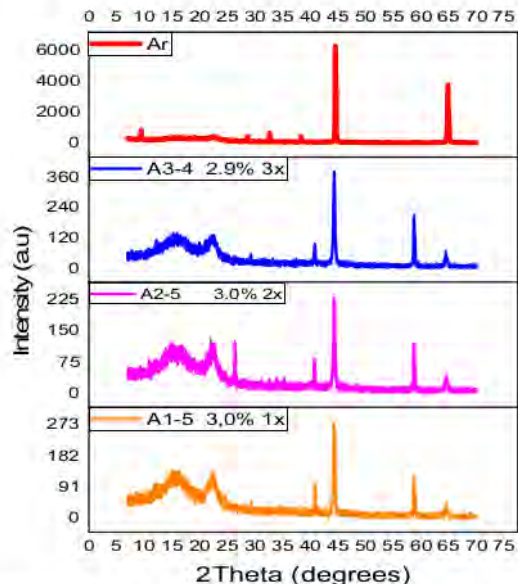
Fig.-2: XRD Diffraction Spectrum Pattern (a) A1-5, (b) A2-5, (c) A3-3 (d) A3-4 and (G) Ar
