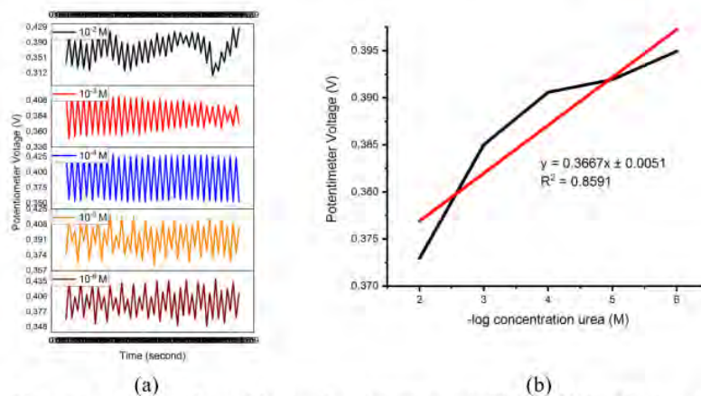
Figure 6. Analysis of variable signal and sensitivity is 36.67 mV/decade, detection range is 10^{-6} - 10^{-2} M and detection limit is 10^{-6} M, R^2 = 85.91\% . B3-4.
