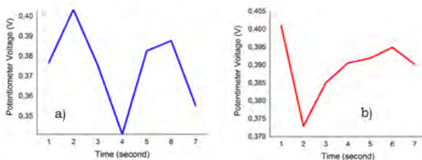
Figure 3. The response time to the potentiometer cell voltage ranged from 10^{-7} - 10^{-1} M urea variation in \text{KH}_2\text{PO}_4 buffer solution with 0.001 M \text{KCl} pH 7.5. B1-4 a), B3-4 b).
