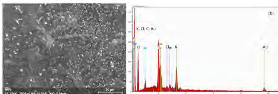
Figure 3. (a) Morphology of SEM M_1 , (b) Spectrum pattern EDS M_1 .
