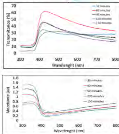
Figure 3: Optical properties of ZnO thin film: (a) transmittance, (b) absorbance. [(\alpha h\nu)]^2 = C_D (h\nu - E_{opt}) (2)
