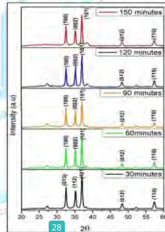
Figure 2: X-ray diffraction spectra of ZnO.
