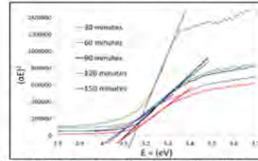
Figure 4: The bandgap of ZnO using Tauc Plot method.
