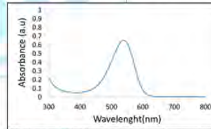
Figure 5: Graph of wavelength Vs absorption of extracted hylocereus polyrhizus dye solution.
