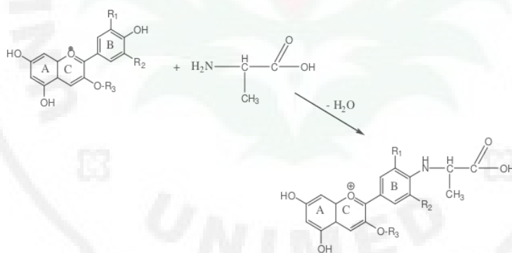
Figure 2. The reaction between anthocyanin and alanine
