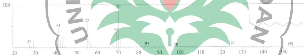
Figure 3 2-decene, 3-methyl
