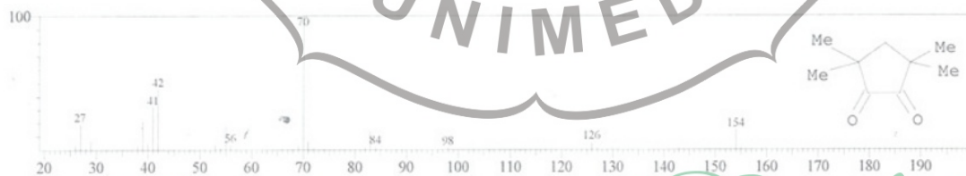
Figure 4 1,2-cyclopentanedione, 3,3,5,5-tetramethyl
