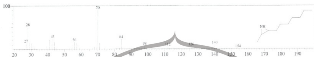
Figure 6 Aziridine, 2-heptyl-3-methyl
