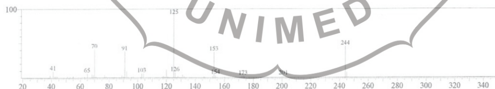
1 Figure 9 3-benzyl-1,4-diaza-2,5-dioxobicyclo[4.3.0]nonane
