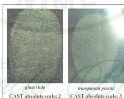
FIGURE 2. Representative photographs of visualised fingerprints on glass slide and transparent plastic using gambir powder (0.250mm).
