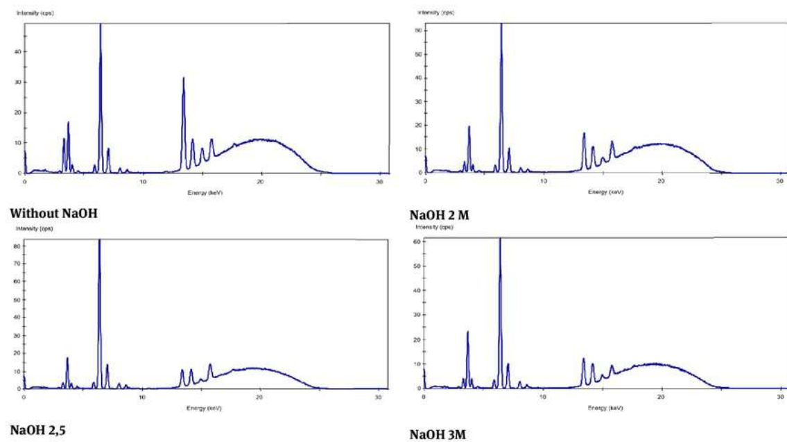
Figure 3: OPBA nanoparticle XRF analysis
