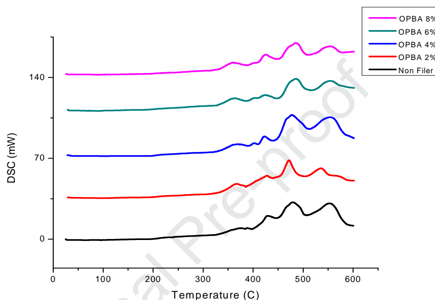
Fig.1. DSC Thermogram of natural rubber compound with OPBA filler (0-8)wt%
