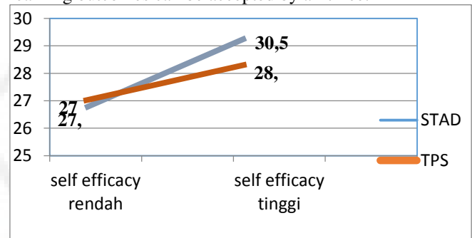
Fig 1. Data Analysis
