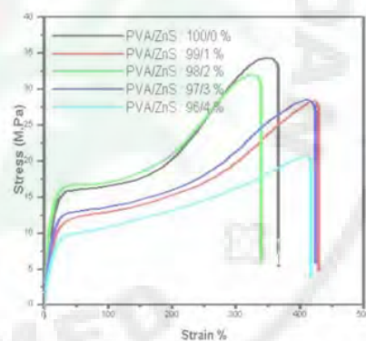
Figure 2. Graph of stress to strain the relationship between the composition of a mixture of several PVA and ZnS nanoparticles.
