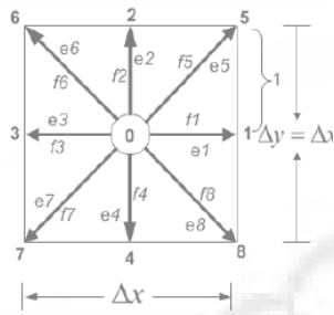
Gambar 2. Distribusi f_i Model D2Q9
