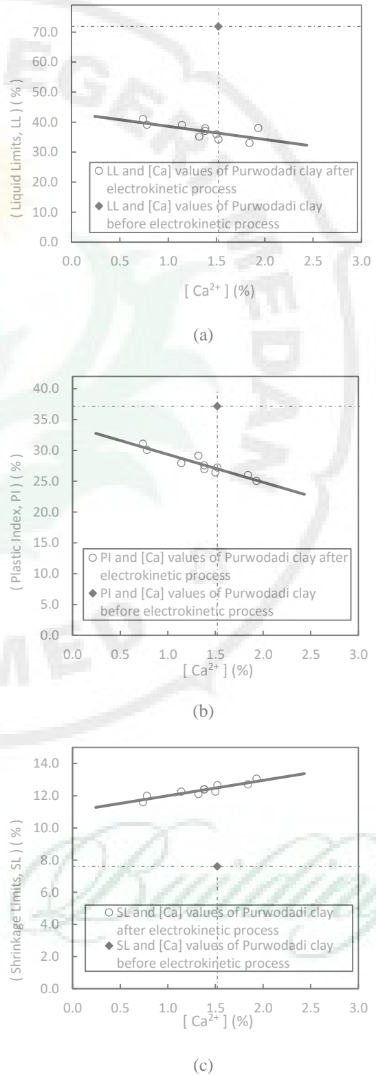
Fig.4 Results testing of propertis clay soil from Purwodadi due of electrokinetic process (a). Liquid Limits, (b). Plastic Index, (c). Shrinkage Limits
