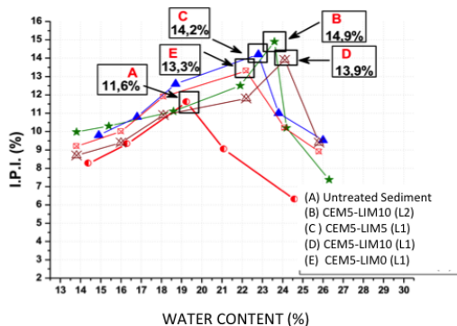
Gambar 1. Hasil percobaan California Bearing Ration
