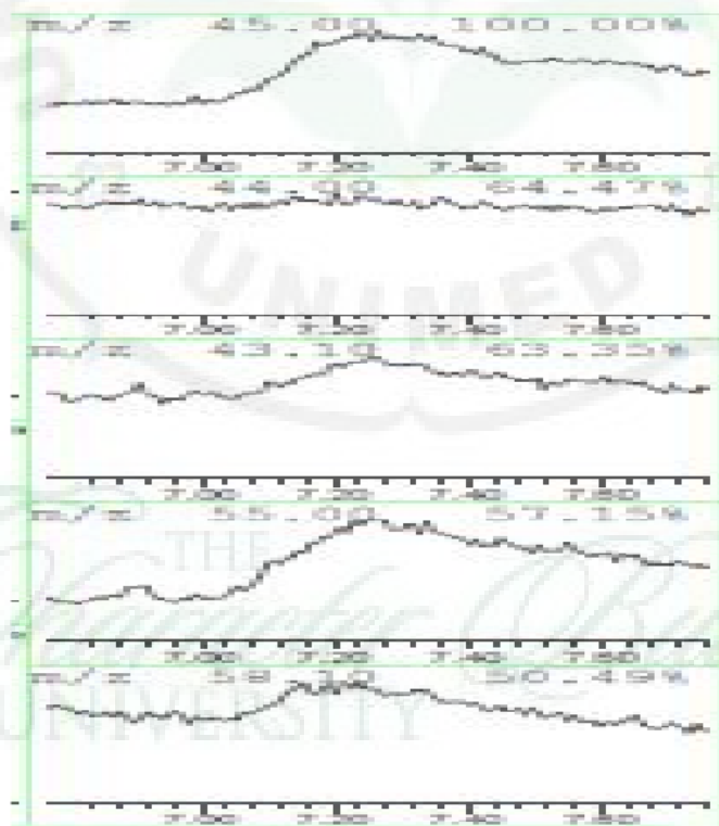
Figure 1. GC-MS profile of the crude leaf extract of P. pubescens
