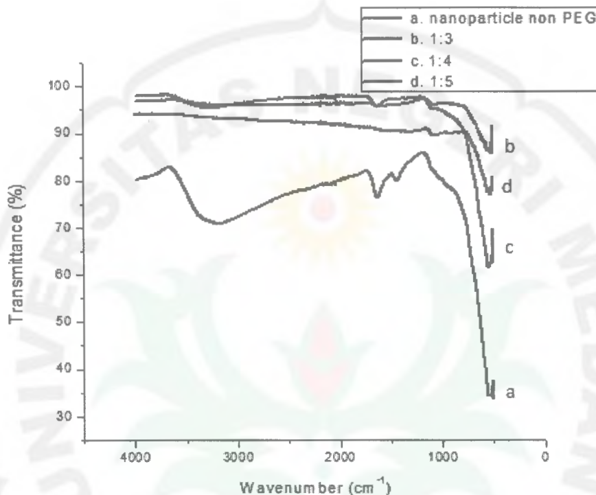
Figure 3 . The results Fe_3O_4 Characterization Using FTIR (a) Without PEG 6000 , (b) 1:3 ,(c) 1:4 ,and (d) 1:5
