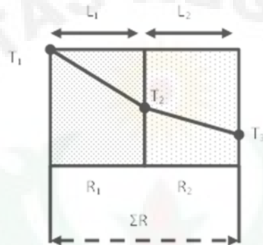
FIGURE 1. Heating Plate Lining Material Structure
