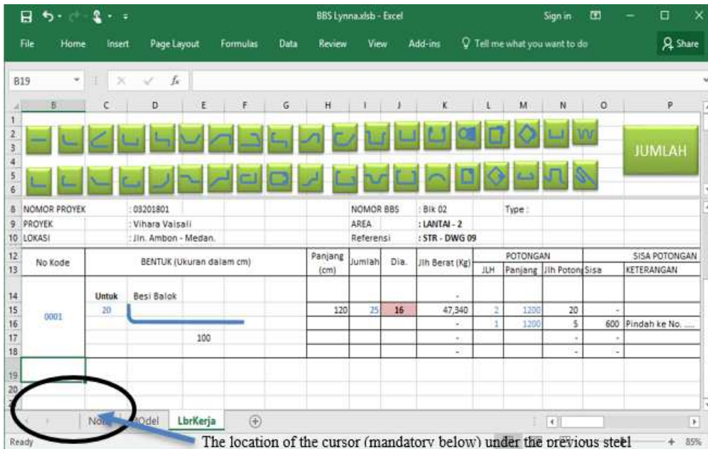
Figure 8 Advanced data input
