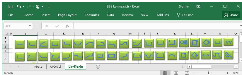
Figure 3 Reinforcement model
