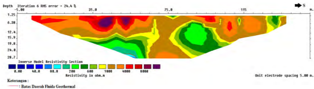
Figure 5. Resistivity section of line 3
