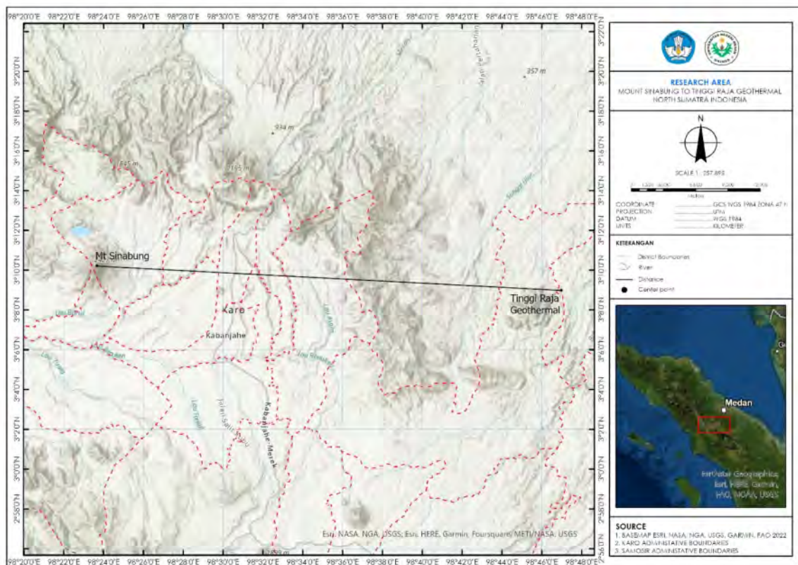
Fig. 2. Research area with a combined geographical location of Mount Sinabung and Tinggi Raja geothermal area, Simalungun District.
