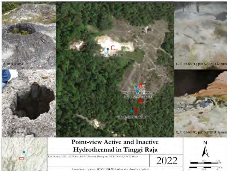
Fig. 5. Point-view (a), (b) inactive hydrothermal spring and (c), (d) active hydrothermal spring in Tinggi Raja.
