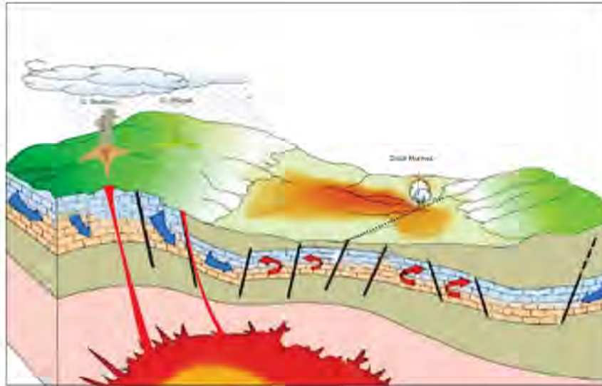
Fig. 8. FMA shows slice of area between Mount Sinabung and Tinggi Raja's geothermal, Dolok Morawa, Simalungun District.
