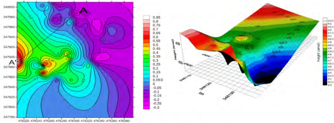
Fig. 6. The distribution of geomagnetic and gravity anomaly in Tinggi Raja.
