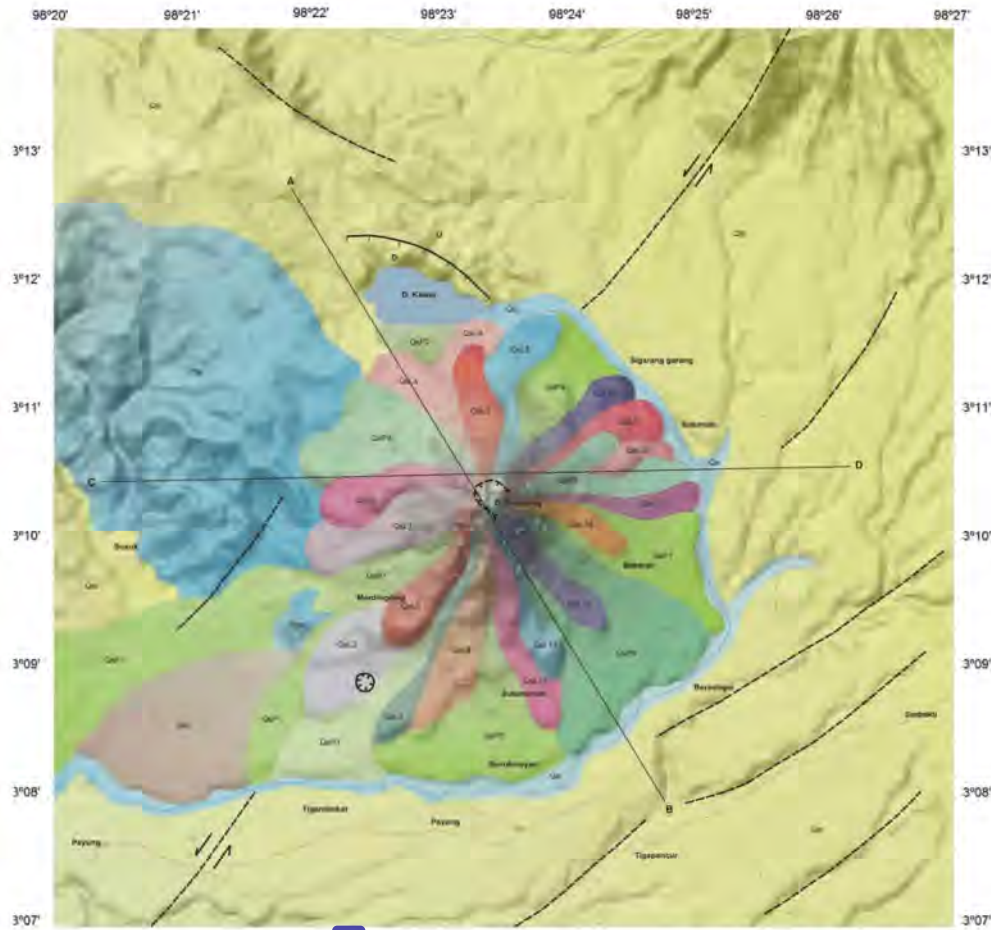
Fig. 3. Geological map of Mount Sinabung, North Sumatra Province (Indrastuti et al., 2019).
