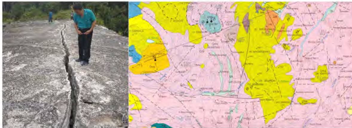
Fig. 7. Inactive faults found in Tinggi Raja and geological map of rocks and faults distribution.
