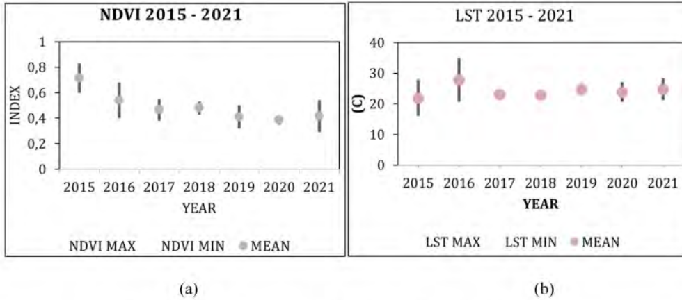
Fig. 4. (a) The distribution of NDVI values (b) LST values from 2015 to 2021 in study area.
