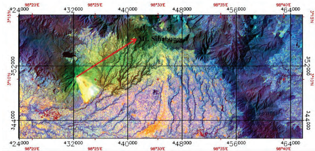
FIGURE 2. Mt. Sinabung in InfraRed Light (Band 10,6,5)
