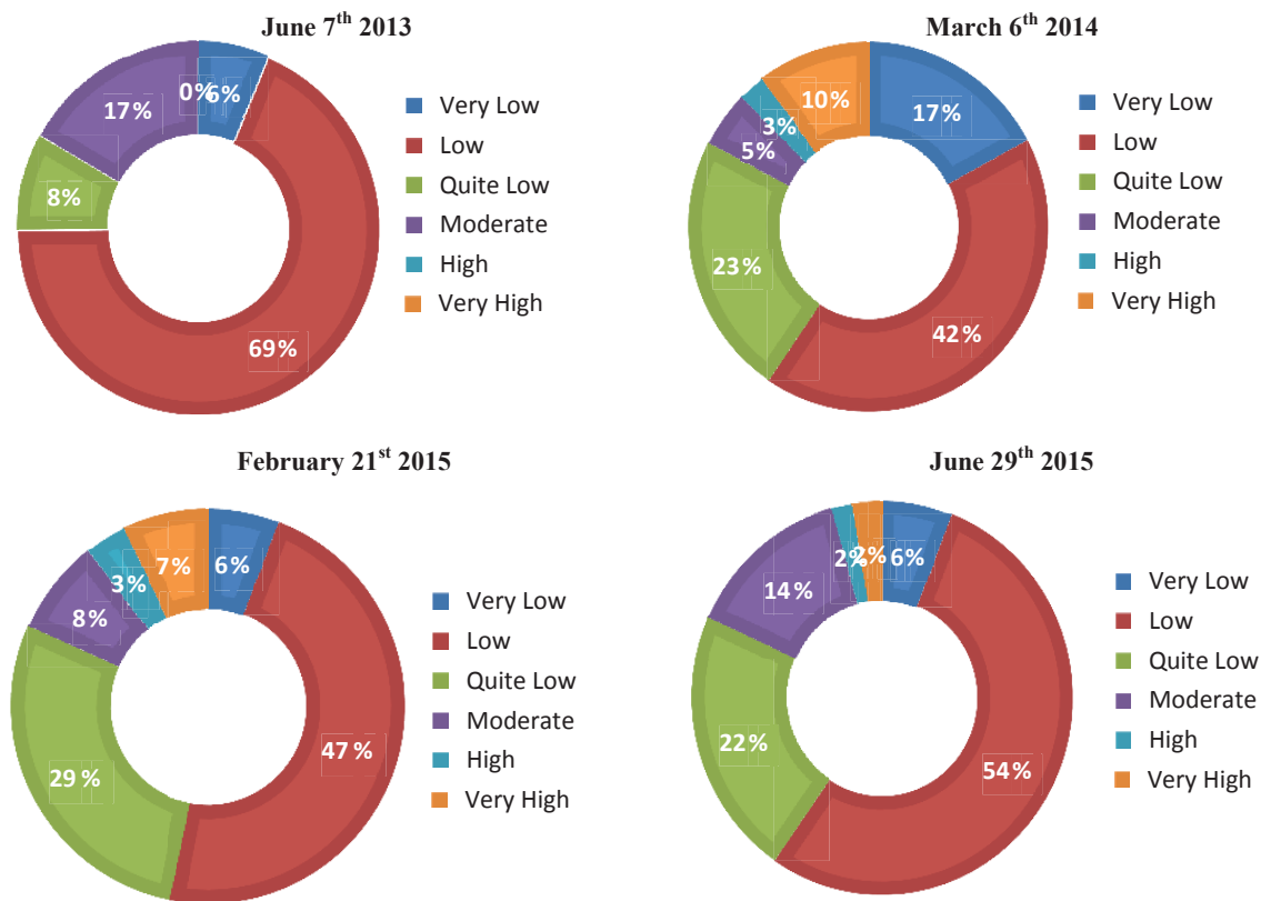
FIGURE 3. Graph for 4 periode of eruption
