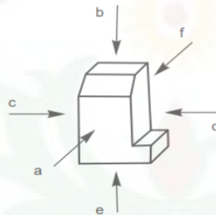
Figure 1. Designation of the Views
