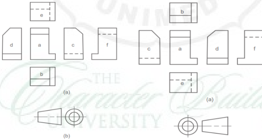
Figure 2. Relative Positions of Six Views in First Angle Projection
