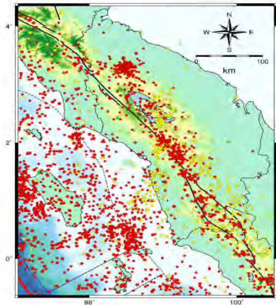
Fig. 1 Seismicity in Northern Sumatra, period 2009 to 2019
