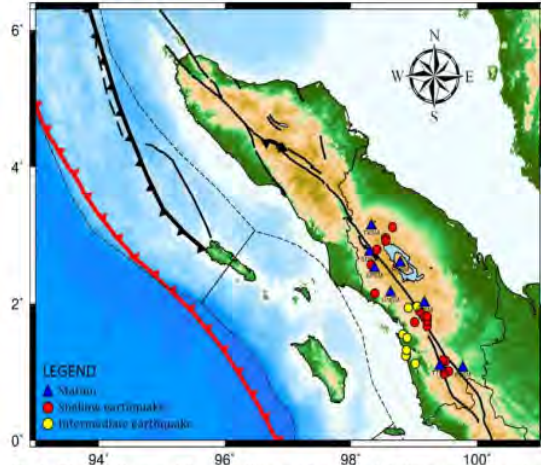
Fig.3. The Shallow and Intermediate earthquake with the new mini region station recorded.
