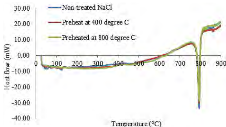
Figure 5. Enlarged DSC graph 2 results
