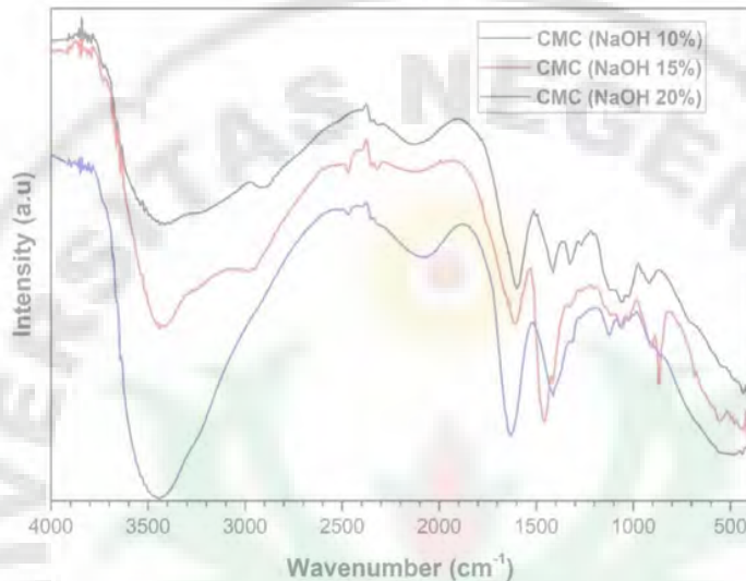
Figure 6. Comparison of FT-IR spectra of CMC synthesized with variations of 10%, 15% and 20% NaOH in the range 4000-400 \text{cm}^{-1} .
