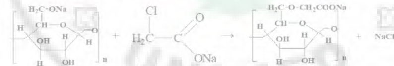
Figure 3. Alkalinization and etherification reaction on CMC formation from BC nata de coco.
