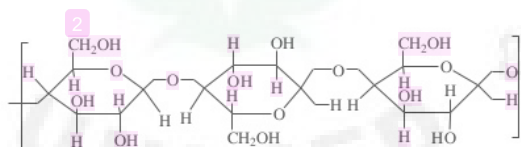
Figure 2. Cellulose structure
