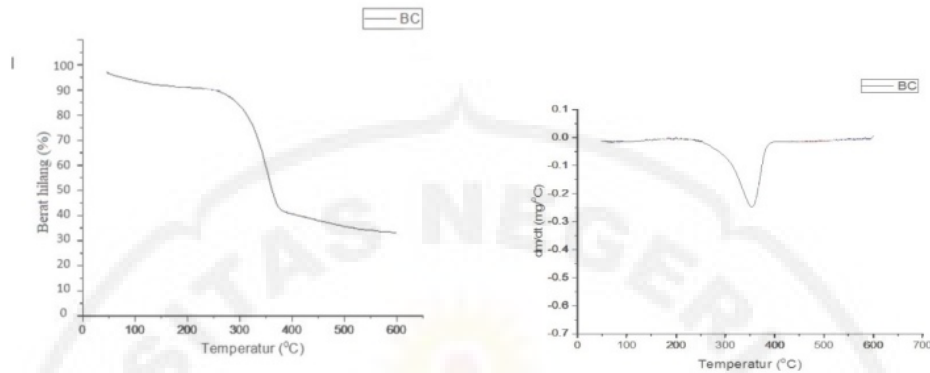
Figure5. TGA graph (a) and DTA graph (b) from BC
