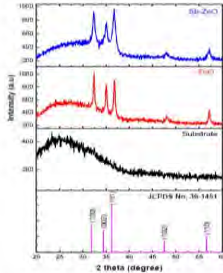
Figure 1. XRD Spectrum of Samples and Substrate
