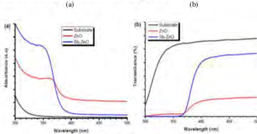
Figure 4. a. Absorbance Spectrum. b. Transmittance Spectrum
