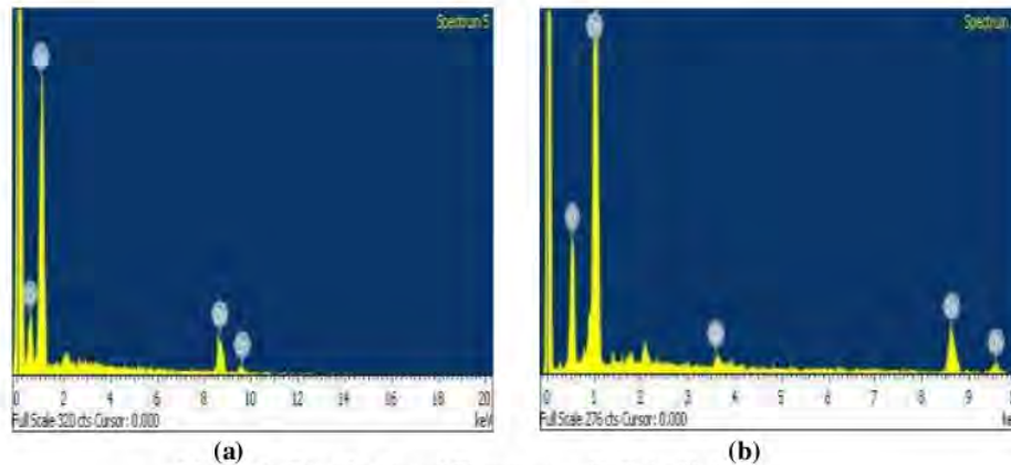
Figure 3. Distribution of Elements: a. ZnO. b. Sb-ZnO
