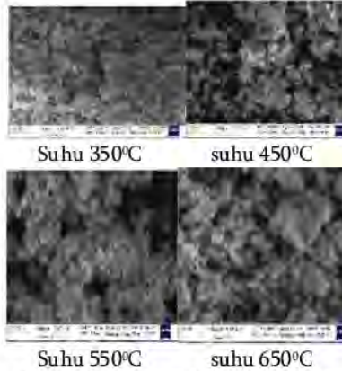
Gambar 3. Analisis Scanning Electron Microscope (SEM)
