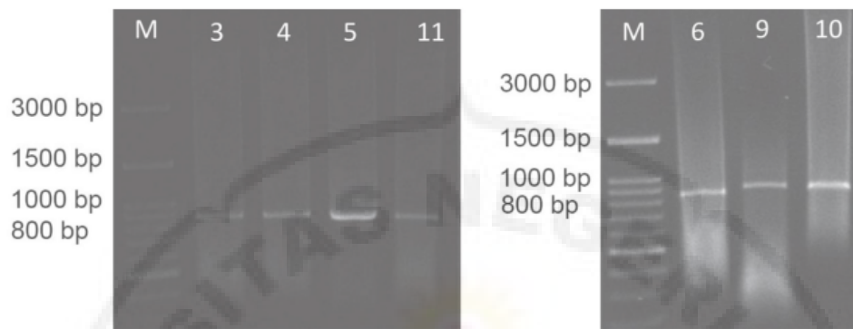
Figure 2: Visualisation of PCR results of matK gene sequences with agarose: (3) South Tapanuli; (4) North Tapanuli; (5) Humbang Hasudutan; (11) Toba Samosir 1; (6) Dairi; (9) Simalungun; (10) Toba Samosir 2.
