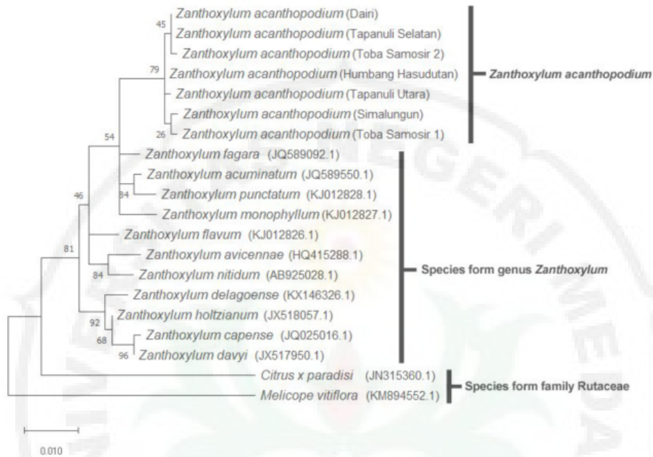
Figure 3: The phylogenetic tree of matK sequence from Z. acanthopodium and outgroup (species in the Zanthoxylum genus and Rutaceae family) as a result of reconstruction using the Maximum Likelihood method based on the kimura-2-parameter model. Branching is analysed with a bootstrap value of 1000x.
