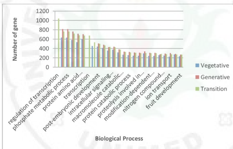
Fig. 4. Chart of GO Categories of Teak
