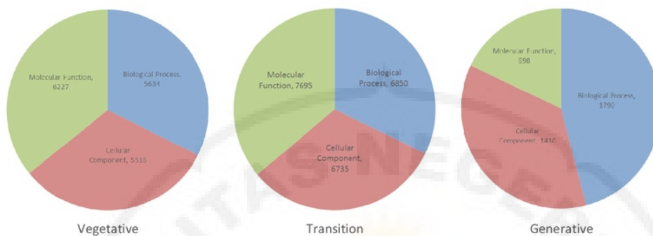
Fig. 4. Chart of GO Categories of Teak
