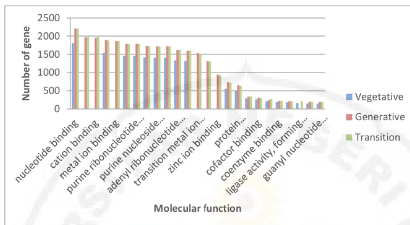
Fig. 5. Histogram of GO Classification of Teak
