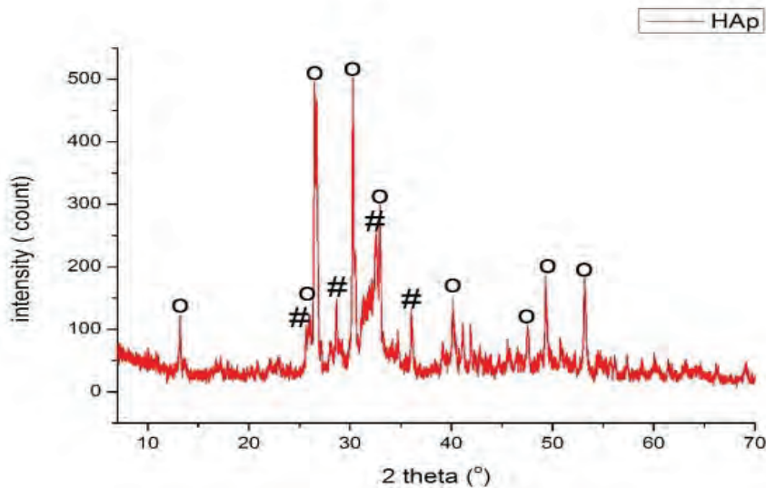
FIGURE 2. Graph of Hydroxyapatite X-Ray Diffraction Pattern
