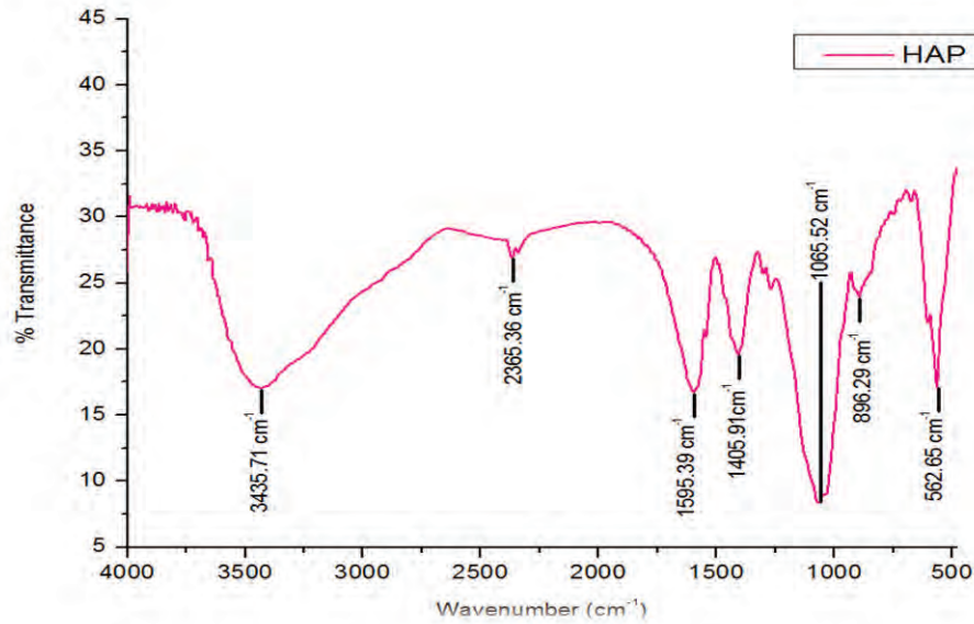
FIGURE 1. Spectrum of Broiler Eggshell Hydroxyapatite
