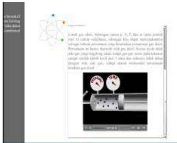
Figure 3. Simulation of how molecules in a gaseous state behave in an enclosed space
