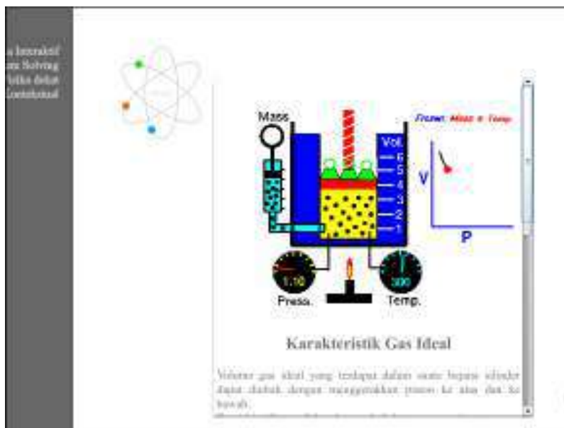
Figure 4. Visualization of Ideal Gas Characteristics
