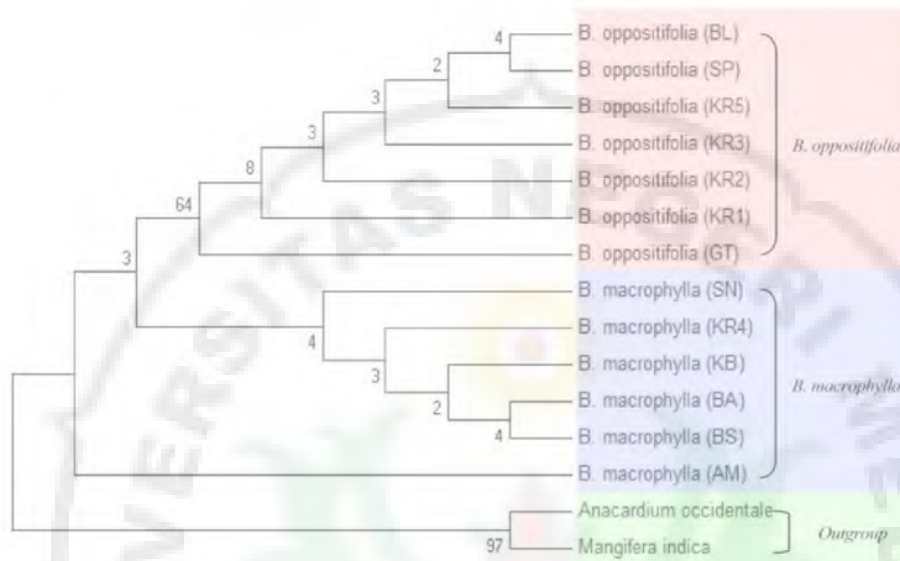
Figure 3. Phylogenetic tree of trnL-F sequences of Bouea and outgroup ( A. occidentale and M. indica ) which was reconstructed using Maximum parsimony methods based on kimura-2-parameter models. Branching analyzed by bootstrap values > 50% of 1000 replicates.
