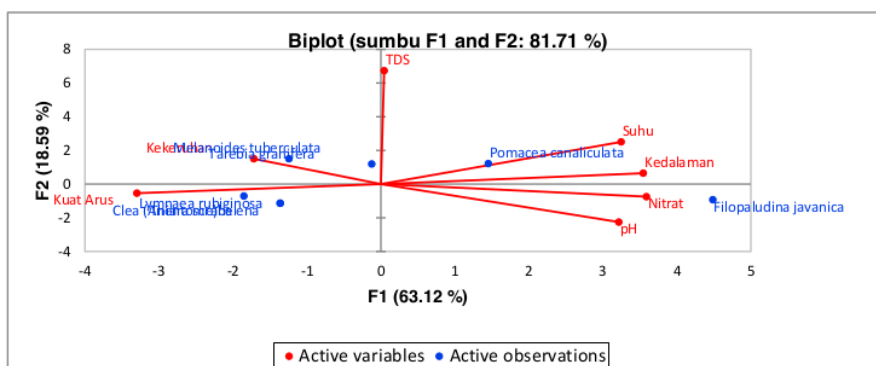
Figure 4. Parameters Affecting Gastropods With PCA Analysis
