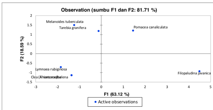
Figure 3. Grouping of Gastropods Based on PCA Analysis
